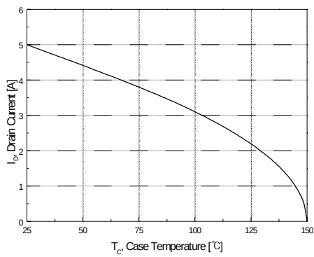
Figure 9-1. Maximum Safe Operating Area for IRF620B
