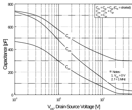
Figure 5. Capacitance Characteristics
