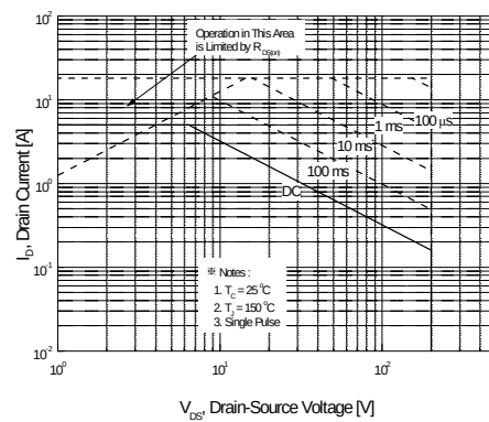
Figure 9-2. Maximum Safe Operating Area for IRFS620B
