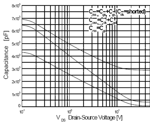
Capacitance Characteristics
