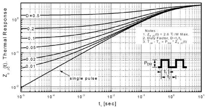
Transient Thermal Response Curve For JCS8N60F
