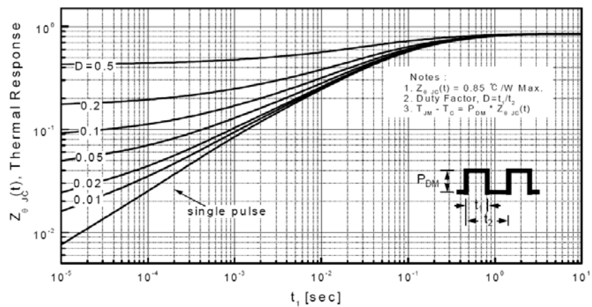
Transient Thermal Response Curve For JCS8N60F
