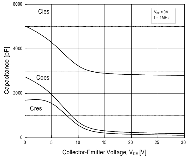
Fig.8 Typical Capacitance
