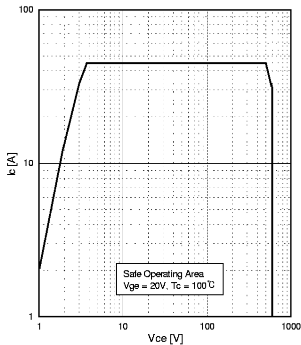
Fig.11 Turn-off SOA
