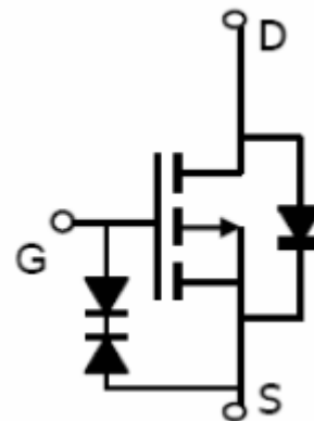
Schematic diagram
