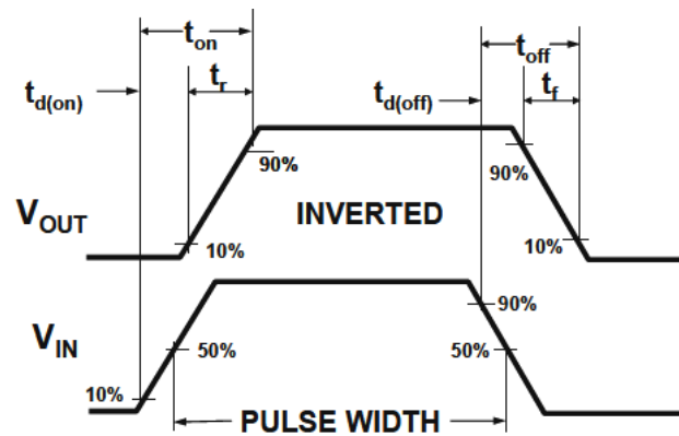
Switching Waveforms
