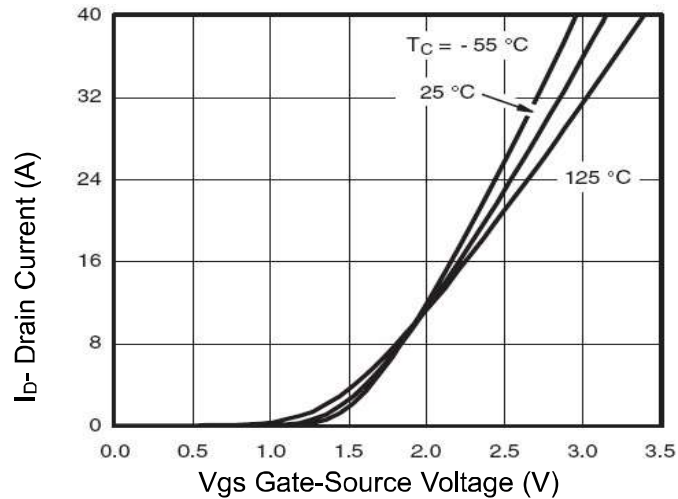
Figure 7 Transfer Characteristics
