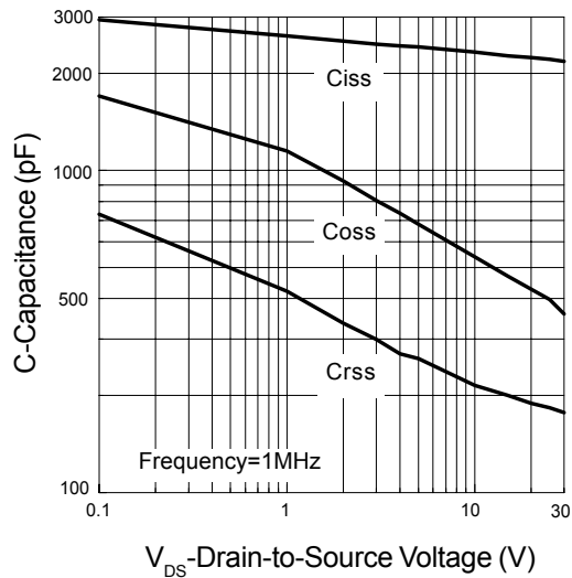
Capacitance Characteristics
