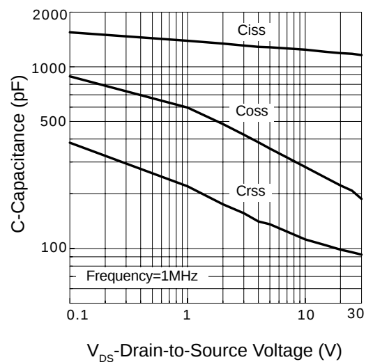
Capacitance Characteristics
