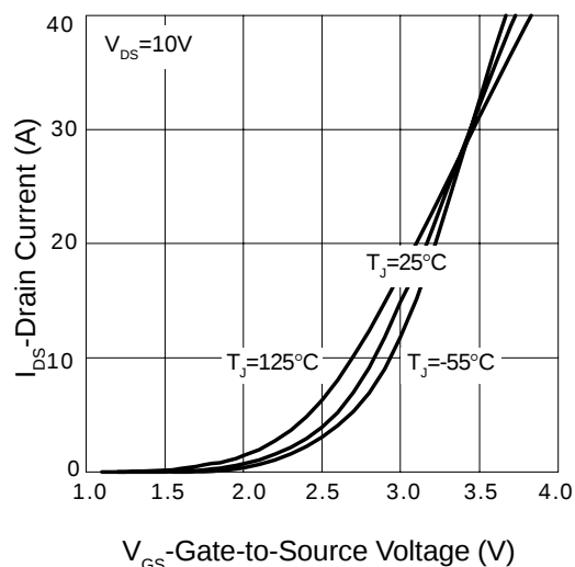
Transfer Characteristics
