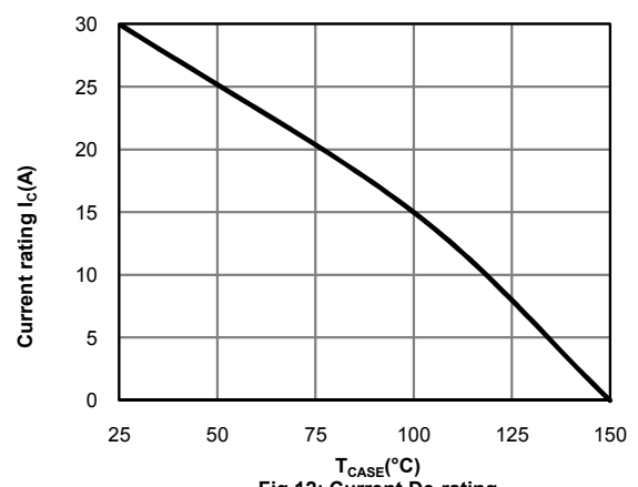
Fig 12: Current De-rating
