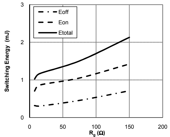
Figure 16: Switching Loss vs. R_g ( T_J=150^\circ\text{C} , V_{GE}=15\text{V} , V_{CE}=400\text{V} , I_C=20\text{A} )
