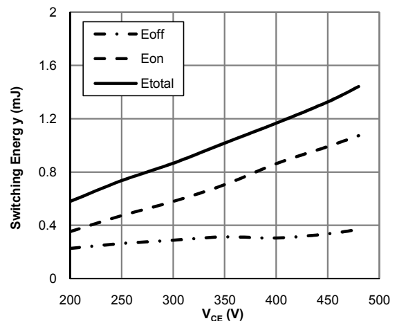
Figure 18: Switching Loss vs. V_{CE} ( T_J=150^\circ\text{C} , V_{GE}=15\text{V} , I_C=20\text{A} , R_g=15\Omega )
