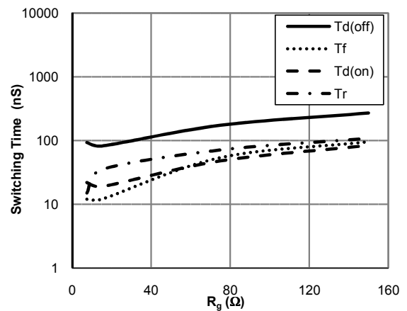
Figure 13: Switching Time vs. R g (T J =150°C, V GE =15V, V CE =400V, I C =20A)
