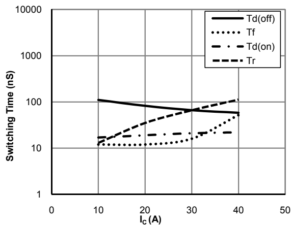
Figure 12: Switching Time vs. I C (T J =150°C, V GE =15V, V CE =400V, R g =15Ω)
