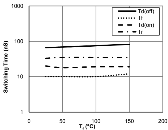
Figure 14: Switching Time vs. T J (V GE =15V, V CE =400V, I C =20A, R g =15Ω)
