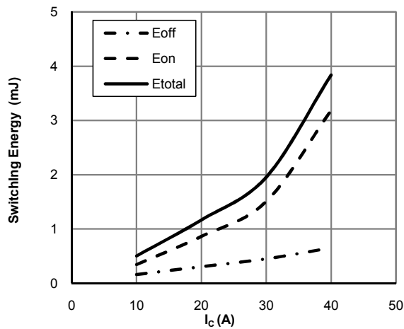
Figure 15: Switching Loss vs. I_C ( T_J=150^\circ\text{C} , V_{GE}=15\text{V} , V_{CE}=400\text{V} , R_g=15\Omega )
