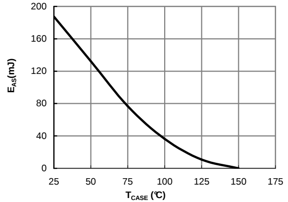
Figure 14: Avalanche energy
