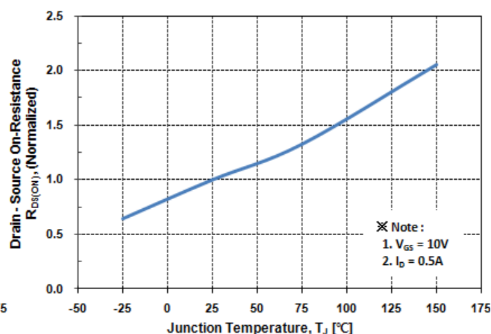
Fig. 8 R_{DS(on)} - T_J
