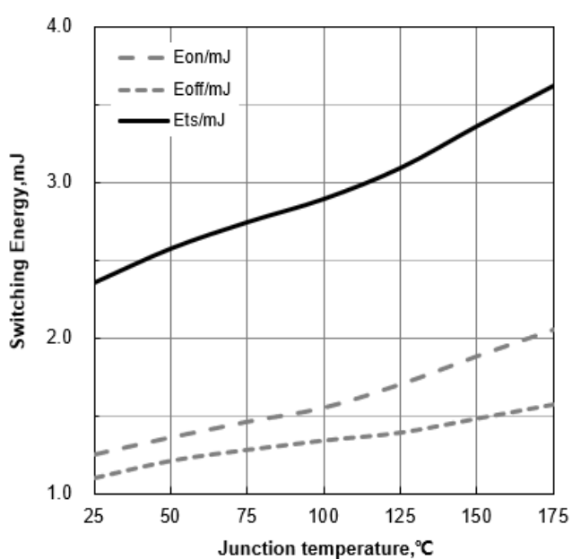
Figure 12. Typical Switching Energy vs Junction Temperature ( V_{CE}=400\text{V} , V_{GE}=15/0\text{V} , I_C=75\text{A} )
