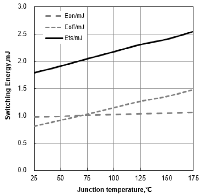
Figure 12. Typical Switching Energy vs Junction Temperature ( V_{CE}=400\text{V} , V_{GE}=15/0\text{V} , I_C=50\text{A} )
