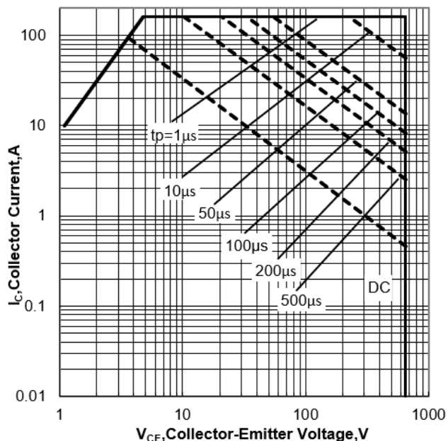
Figure 1. Forward Bias Safe Operating Area for TO247/TO3PF/TO3PN
