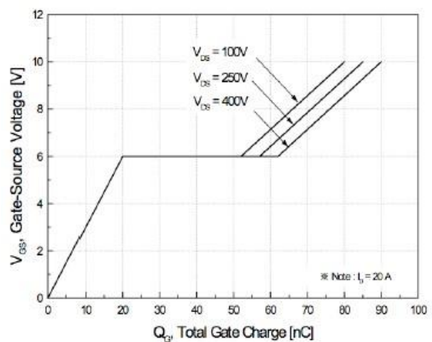
FIG.6-GATE CHARGE CHARACTERISTICS
