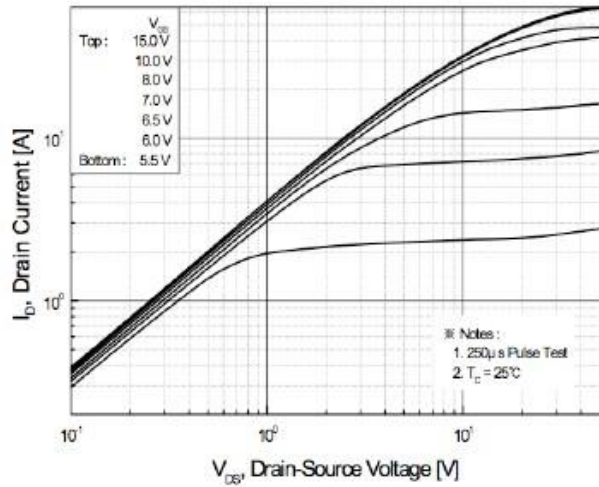
FIG.1-ON REGION CHARACTERISTICS
