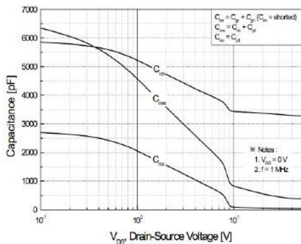
FIG.5-CAPACITANCE CHARACTERISTICS
