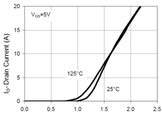
Figure 7 Transfer Characteristics
