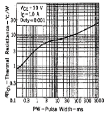
THERMAL RESISTANCE vs. PULSE WIDTH
