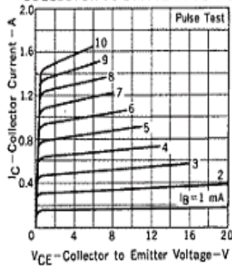
COLLECTOR CURRENT vs. COLLECTOR TO EMITTER VOLTAGE
