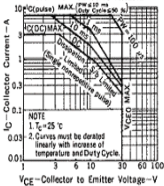
SAFE OPERATING AREAS
