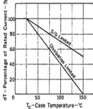
DERATING CURVES FOR ALL TYPES
