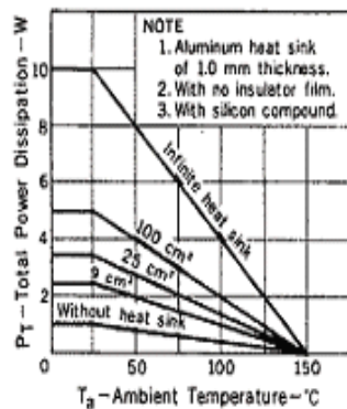
TOTAL POWER DISSIPATION vs. AMBIENT TEMPERATURE
