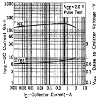
DC CURRENT GAIN, BASE TO EMITTER VOLTAGE vs. COLLECTOR CURRENT
