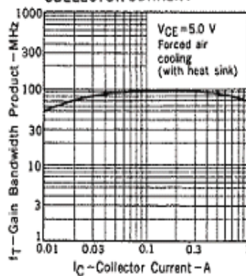
GAIN BANDWIDTH PRODUCT vs. COLLECTOR CURRENT
