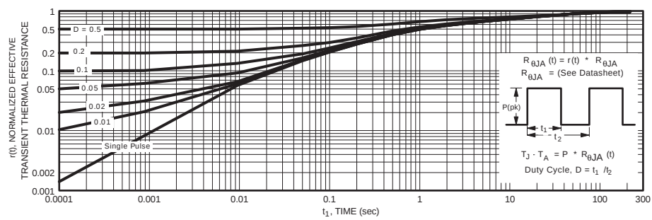
Figure 14. 2N7002VGP Transient Thermal Response Curve
