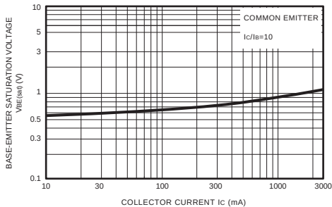
Figure 6. V_{BE(sat)} - I_c
