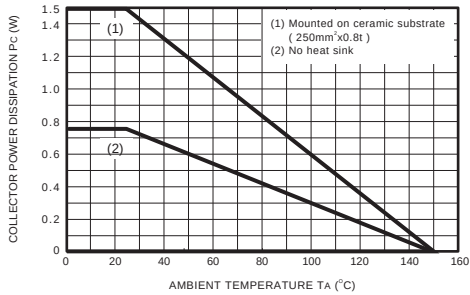
Figure 4. P_c - T_a
