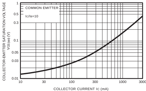
Figure 5. V_{CE(sat)} - I_c
