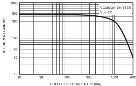
Figure 3. h_{FE} - I_c
