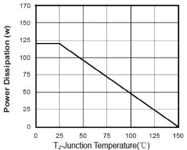
Figure 10 Power De-rating
