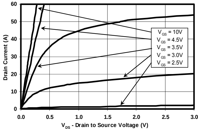
Figure 2: Saturation Characteristics
