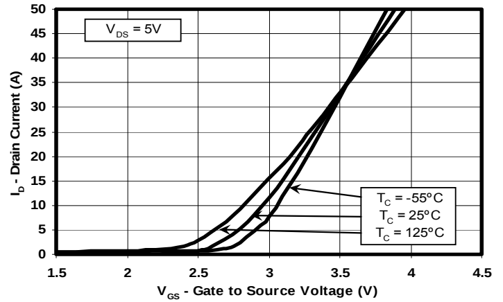
Figure 3: Transfer Characteristics
