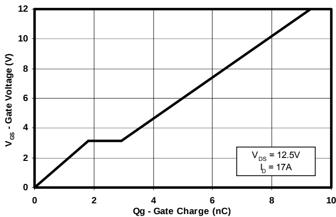
Figure 4: Gate Charge
