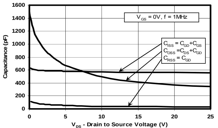
Figure 5: Capacitance
