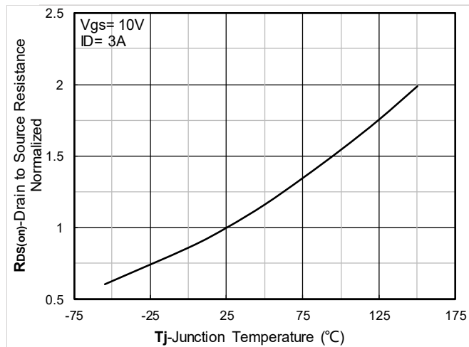
Figure 6. Normalized On-Resistance
