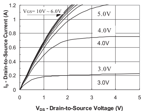
FIG.1- Output Characteristic
