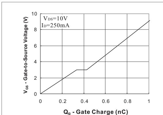
Fig.7 - Gate Charge
