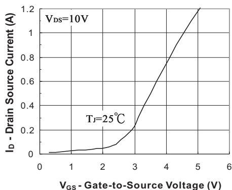
FIG.2- Transfer Characteristic
