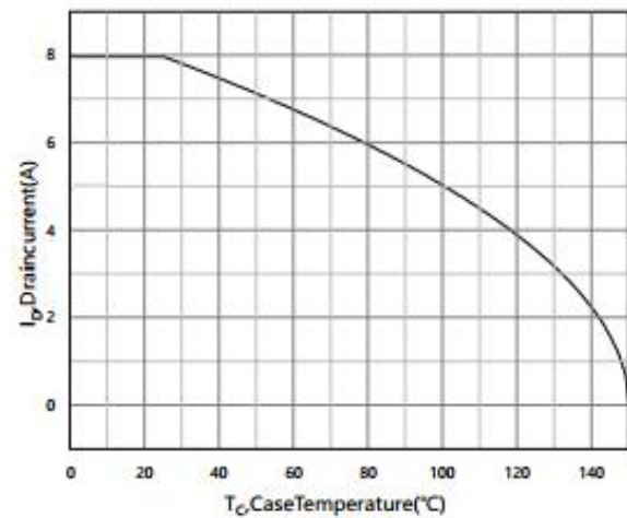
Figure 10. Drain current
