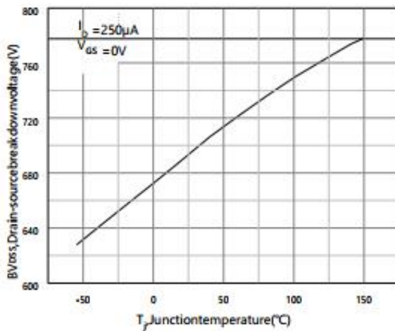
Figure5.Drain-source breakdown voltage
