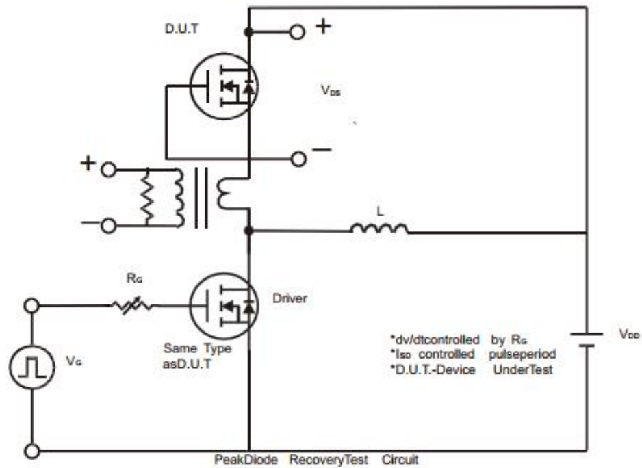
PeakDiodeRecoverydv/dtTestCircuit&Waveform
