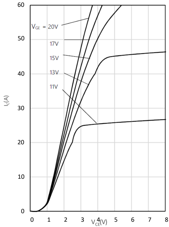
Fig. 3 Output characteristics
