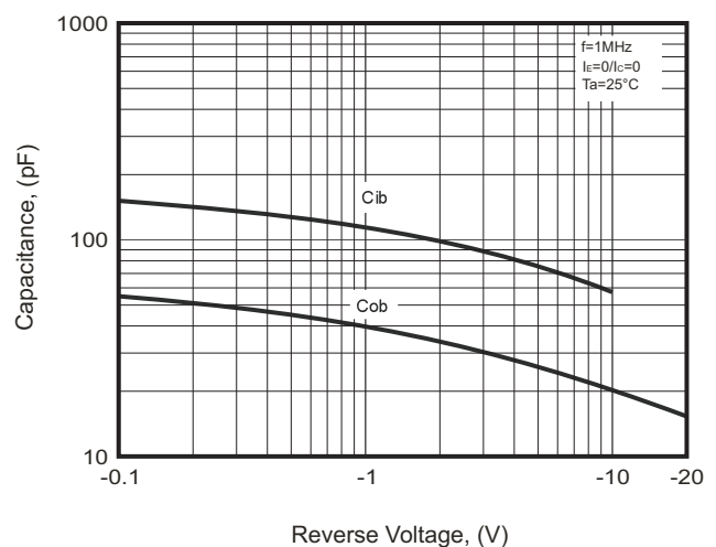
Fig.6 - C_{ob}/C_{ib} — V_{CB}/V_{EB}
