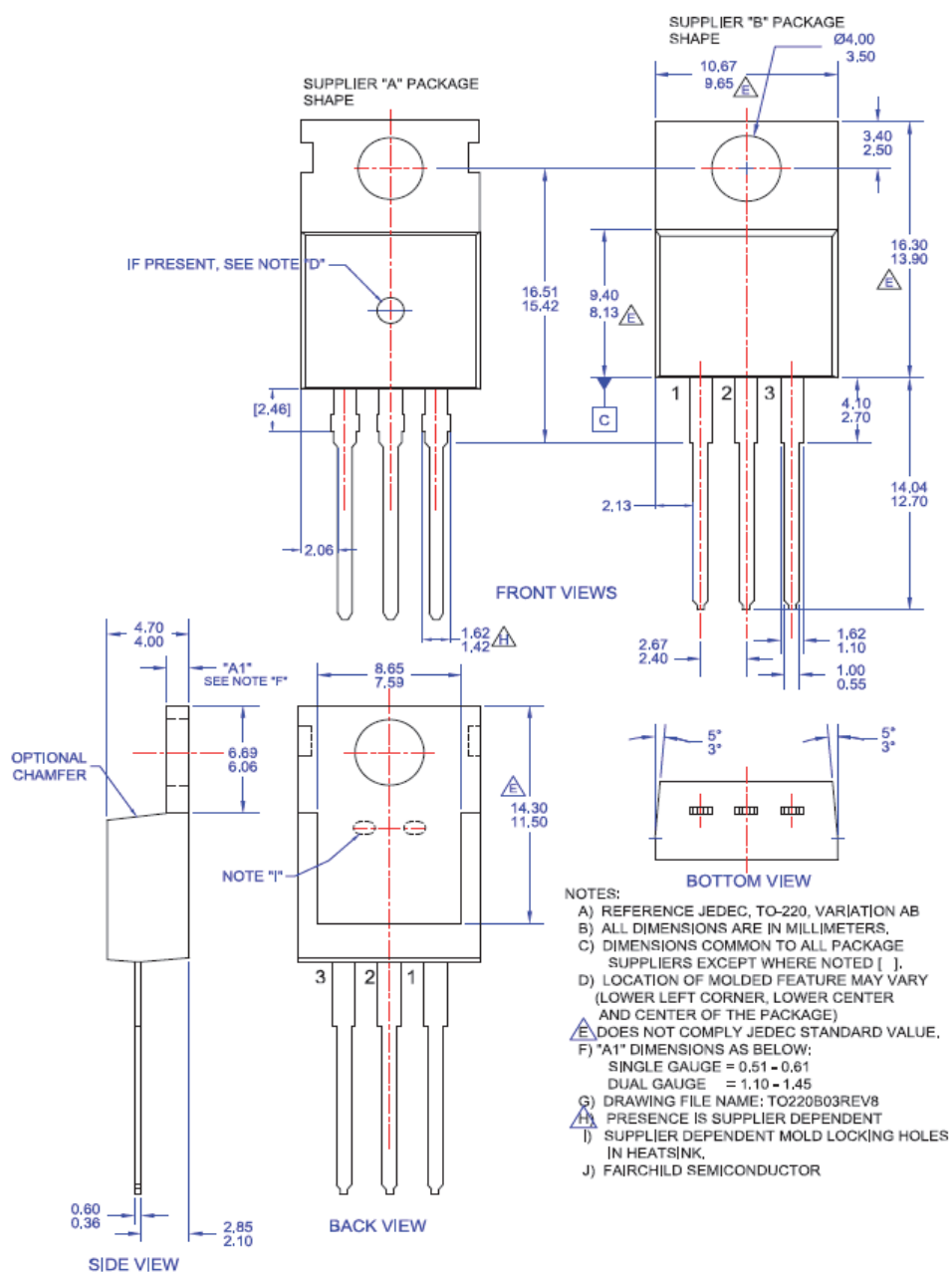
Figure 17. TO-220, Molded, 3Lead, Jedec Variation AB
