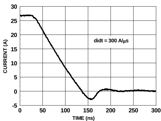
Figure 27. FDMS3606S SyncFET™ body diode reverse recovery characteristic
