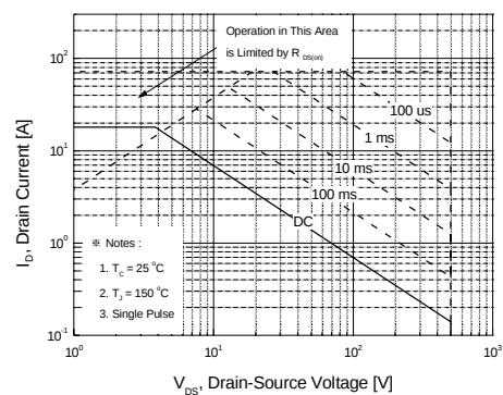
Figure 9-2. Maximum Safe Operating Area for FQP18N50V2
