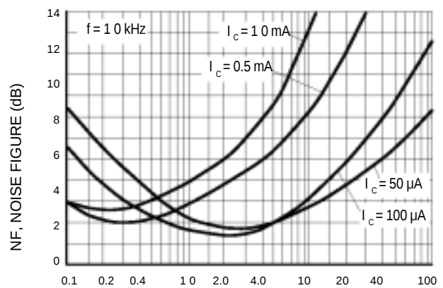
Figure 8. Noise Figure
