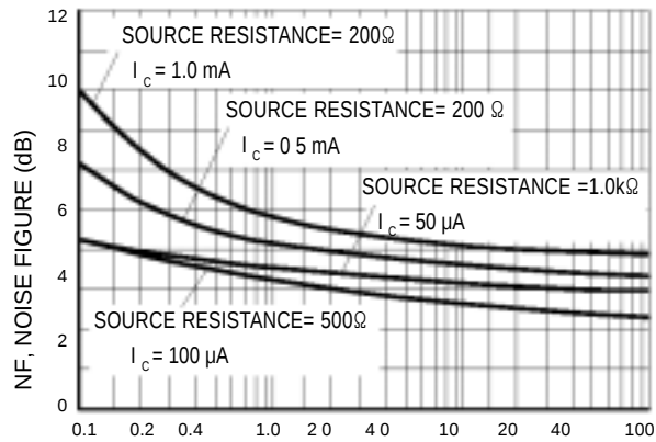
Figure 7. Noise Figure
