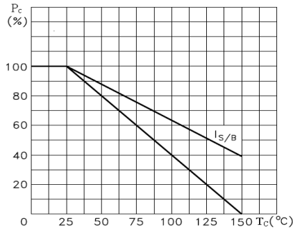
Pc-Tc
