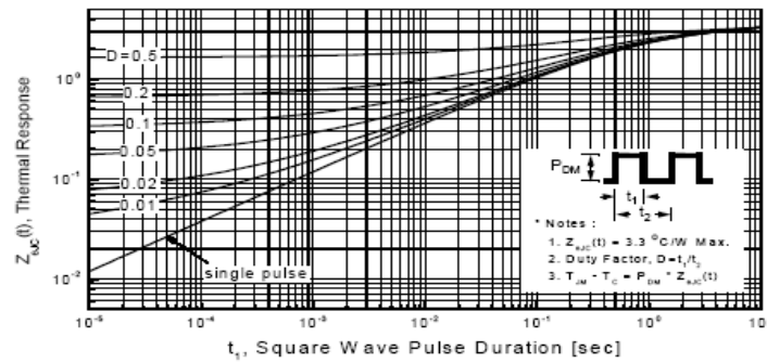
Figure 11-2. Transient Thermal Response Curve for 16N50F
