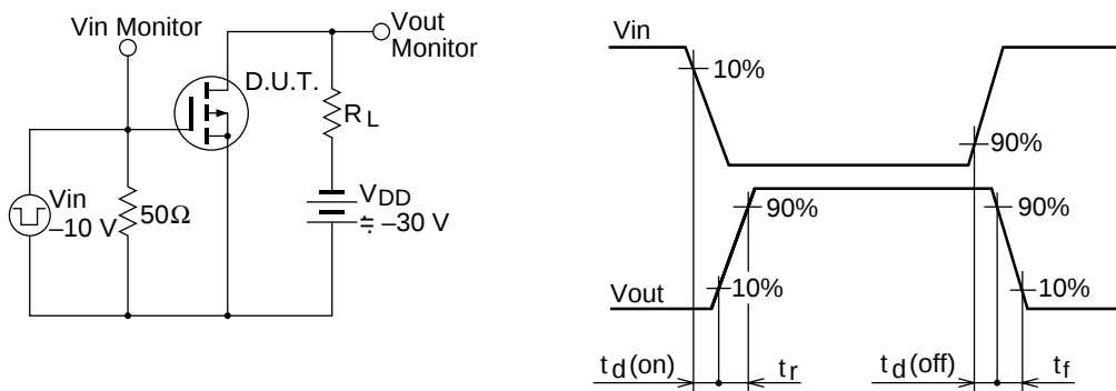
Switching Time Test Circuit Waveform
