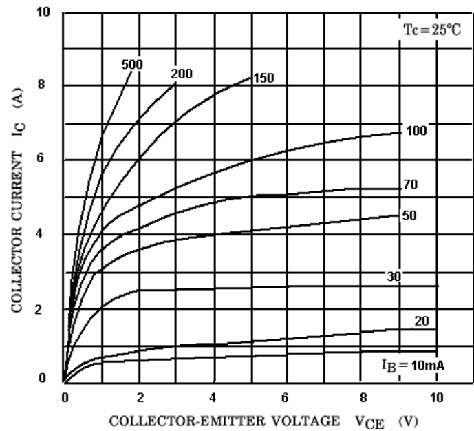
Fig.3 Static Characteristic
