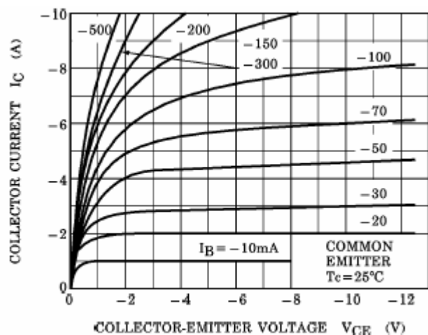
Fig.3 Static Characteristic
