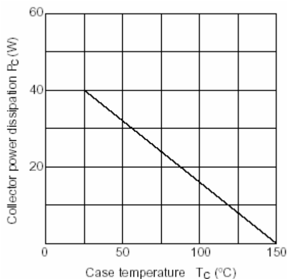
Fig.4 Power Derating
