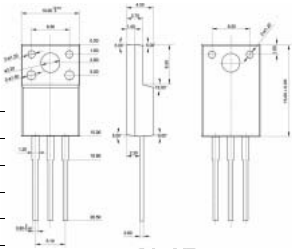
TO-220F
