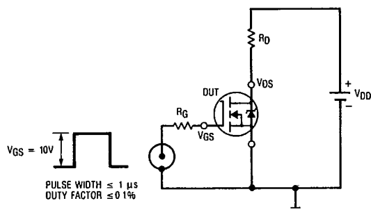
Fig. 15a — Switching Time Test Circuit
