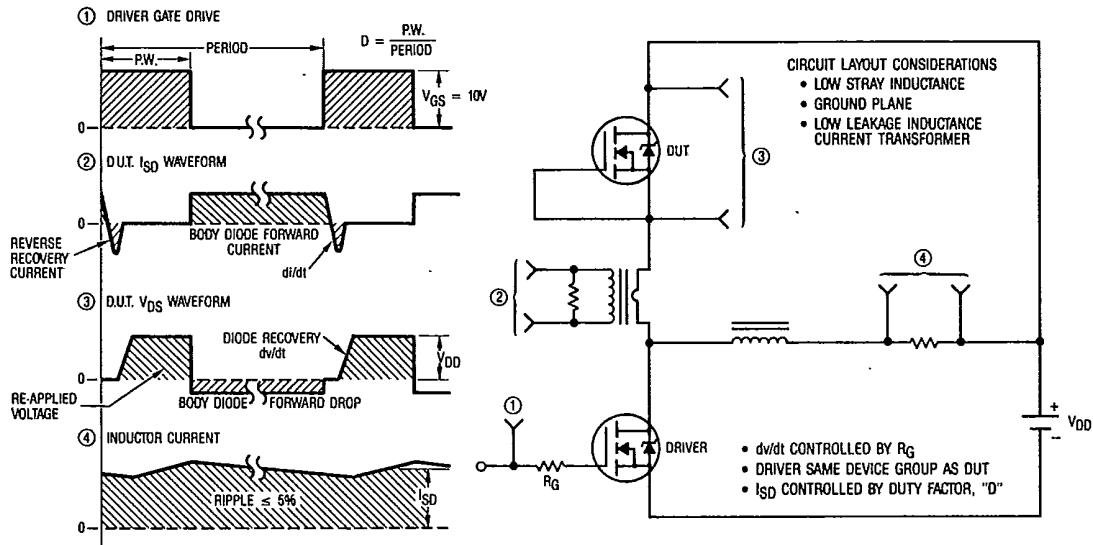
Fig. 17 — Peak Diode Recovery dv/dt Test Circuit
