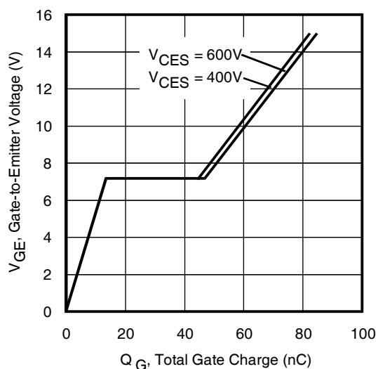
Fig. 18 - Typical Gate Charge vs. V_{GE} I_{CE} = 20A ; L = 2.4mH
