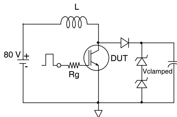
Fig.C.T.2 - RBSOA Circuit
