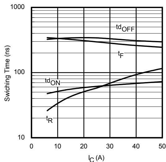
Fig. 15 - Typ. Switching Time vs. I_C T_J = 150^\circ\text{C} ; L = 0.62\text{mH} ; V_{CE} = 600\text{V} ; R_G = 10\Omega ; V_{GE} = 15\text{V}
