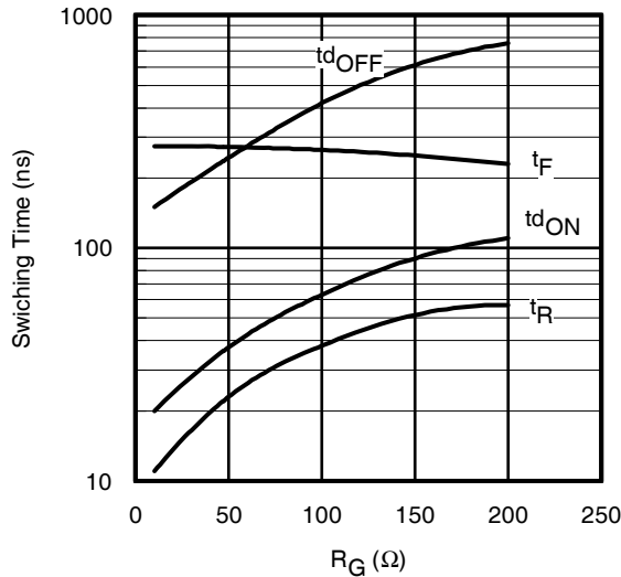
Fig. 15 - Typ. Switching Time vs. R_G T_J = 150^\circ\text{C} ; L = 1\text{mH} ; V_{CE} = 400\text{V} ; I_{CE} = 8\text{A} ; V_{GE} = 15\text{V}
