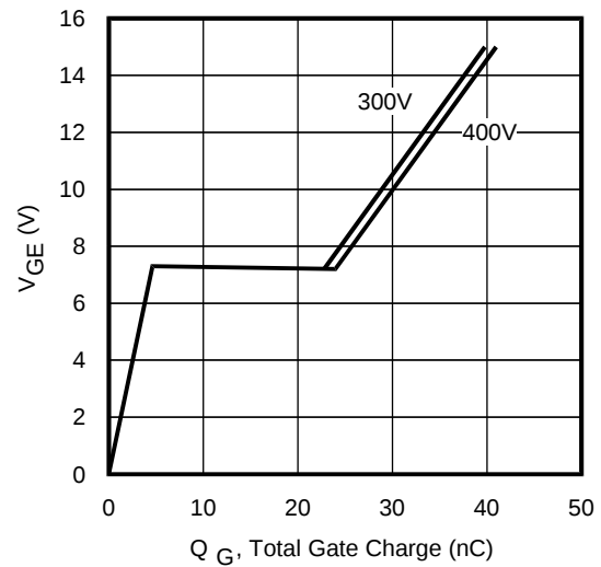
Fig. 23 - Typical Gate Charge vs. V_{GE} I_{CE} = 10A ; L = 2500\mu H
