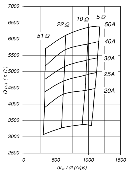
Fig.20 - Typical Diode Q_{RR}
