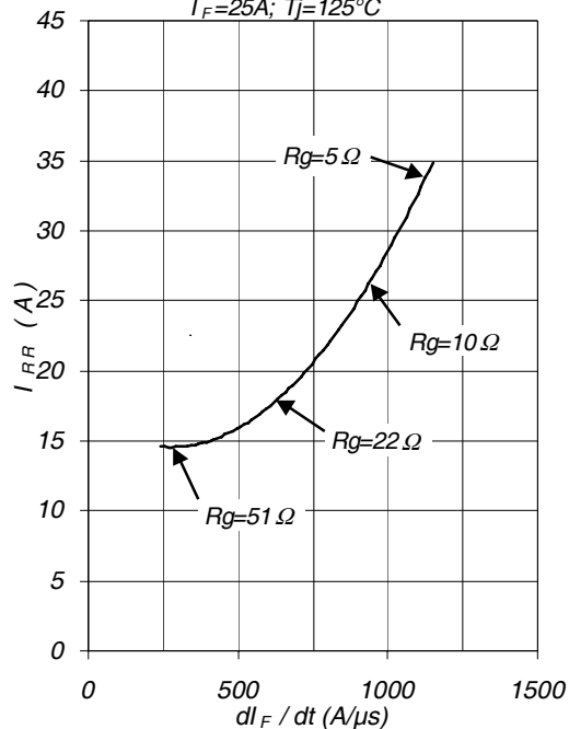
Fig.19 - Typical Diode I_{RR} vs dI_F/dt
