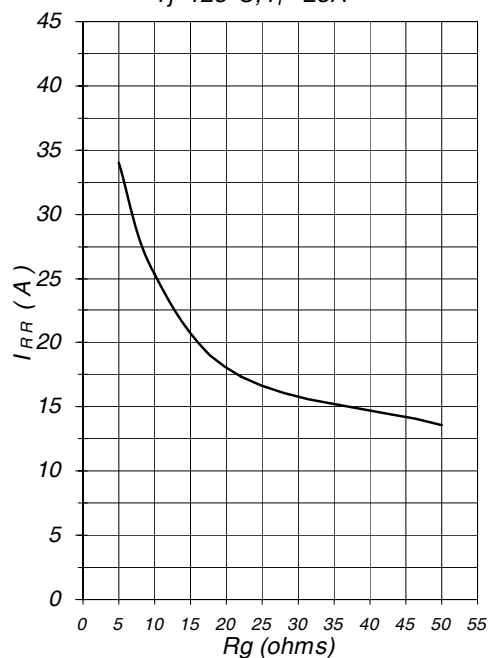
Fig.18 - Typical Diode I_{RR} vs R_g
