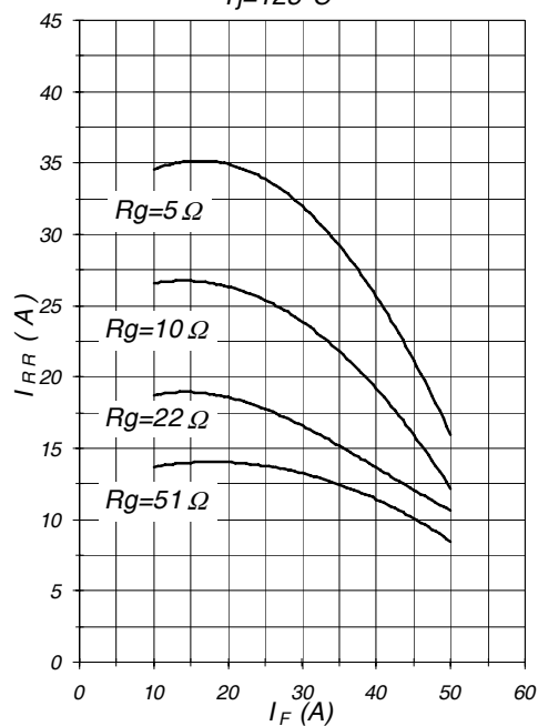
Fig.17 - Typical Diode I_{RR} vs I_F
