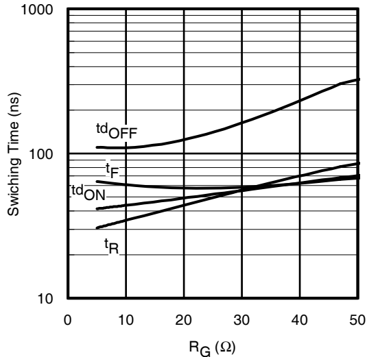
Fig. 15 - Typ. Switching Time vs. R_G T_J = 175^\circ\text{C} ; L = 210\mu\text{H} ; V_{CE} = 400\text{V} ; I_{CE} = 35\text{A} ; V_{GE} = 15\text{V}
