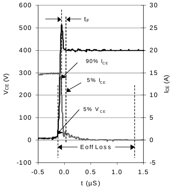
WF.1- Typ. Turn-off Loss @ T_J = 150^\circ C using CT.4
