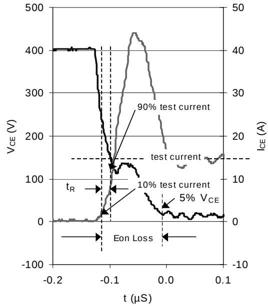
WF.2- Typ. Turn-on Loss @ T_J = 150^\circ C using Fig. CT.4
