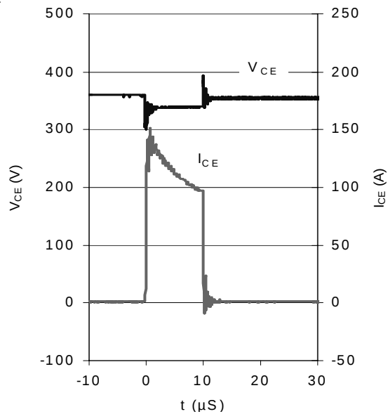
WF.4- Typ. Short Circuit @ T_J = 150^\circ C using CT.3
