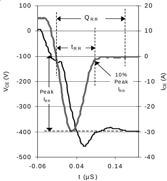
WF.3- Typ. Reverse Recovery @ T_J = 150^\circ C using CT.4
