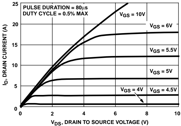
FIGURE 6. SATURATION CHARACTERISTICS
