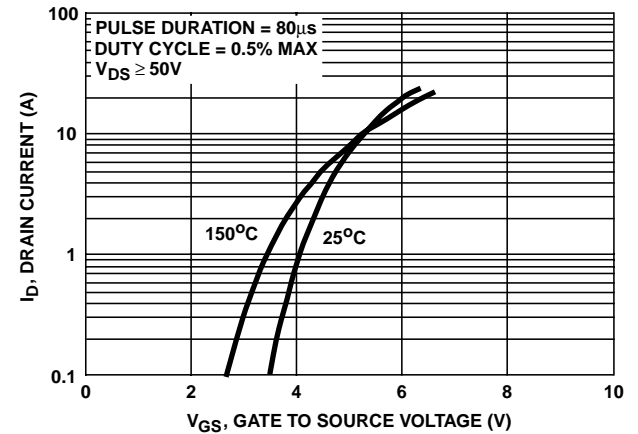
FIGURE 7. TRANSFER CHARACTERISTICS
