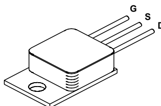
TO-254AA
