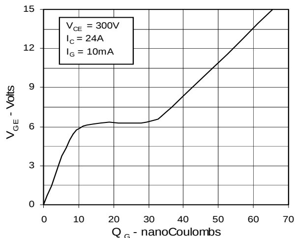
Fig. 14. Gate Charge
